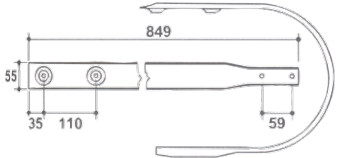
F9381320 GUIDE PLATE KRONE 125
