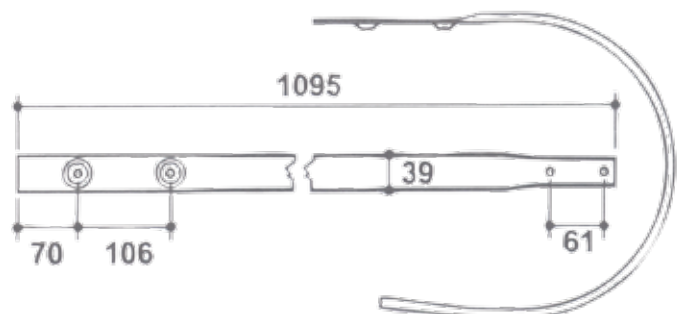
F9383110 OUTER GUIDE PLATE KRONE ROUND PACK
